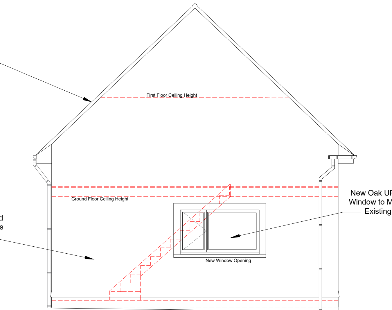
East Elevation
