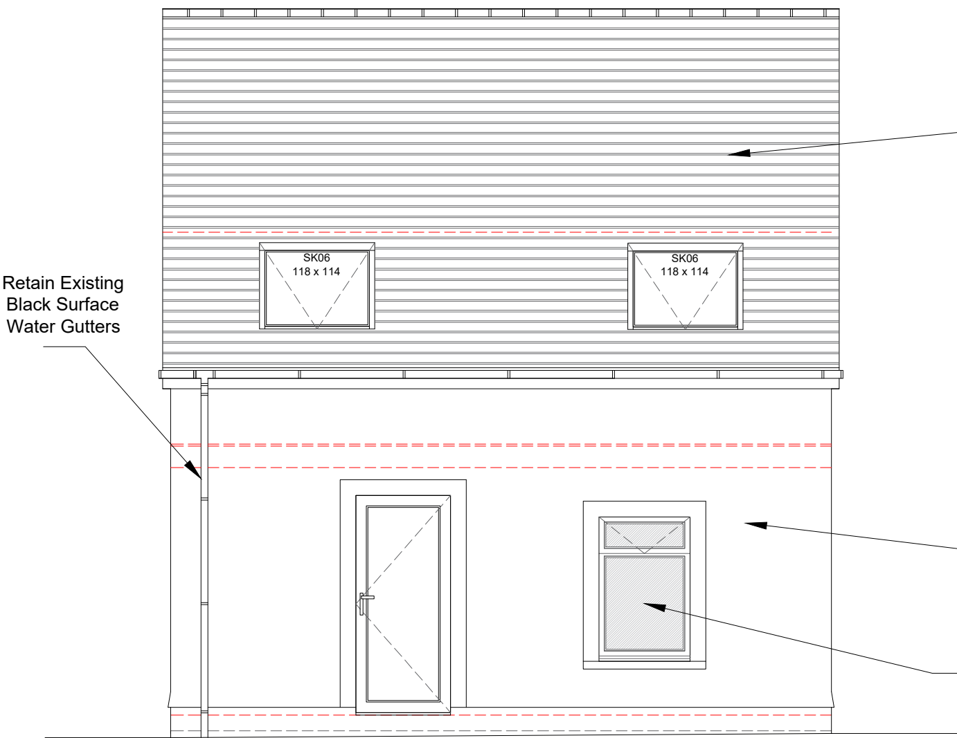
North Elevation
